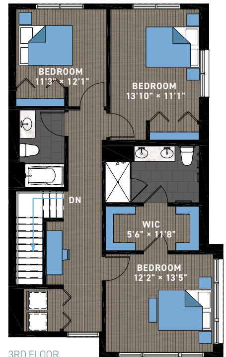
3RD FLOOR 1,080 SF
